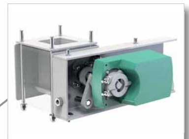
Abrasive control valve to regulate the quantity of the abrasive
