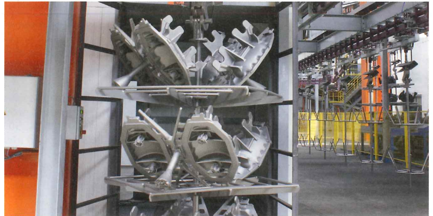
Castings on a hanger on their way to the blasting machine (Photo: AGTOS)
